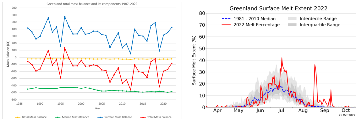
Figure 10: (left) Components of the total mass balance of the Greenland Ice Sheet 1987-2022. Blue: Surface mass balance (SMB), green: marine mass balance (MMB), orange: basal mass balance (BMB), red: total mass balance (TMB), the sum of SMB, MMB and BMB. Mankoff et al. (2021), updated and redrawn by M. Stendel. (right) Greenland Ice Sheet melt extent, 2022.. Image and analysis courtesy of Thomas Mote, U.S. National Snow and Ice Data Center.
